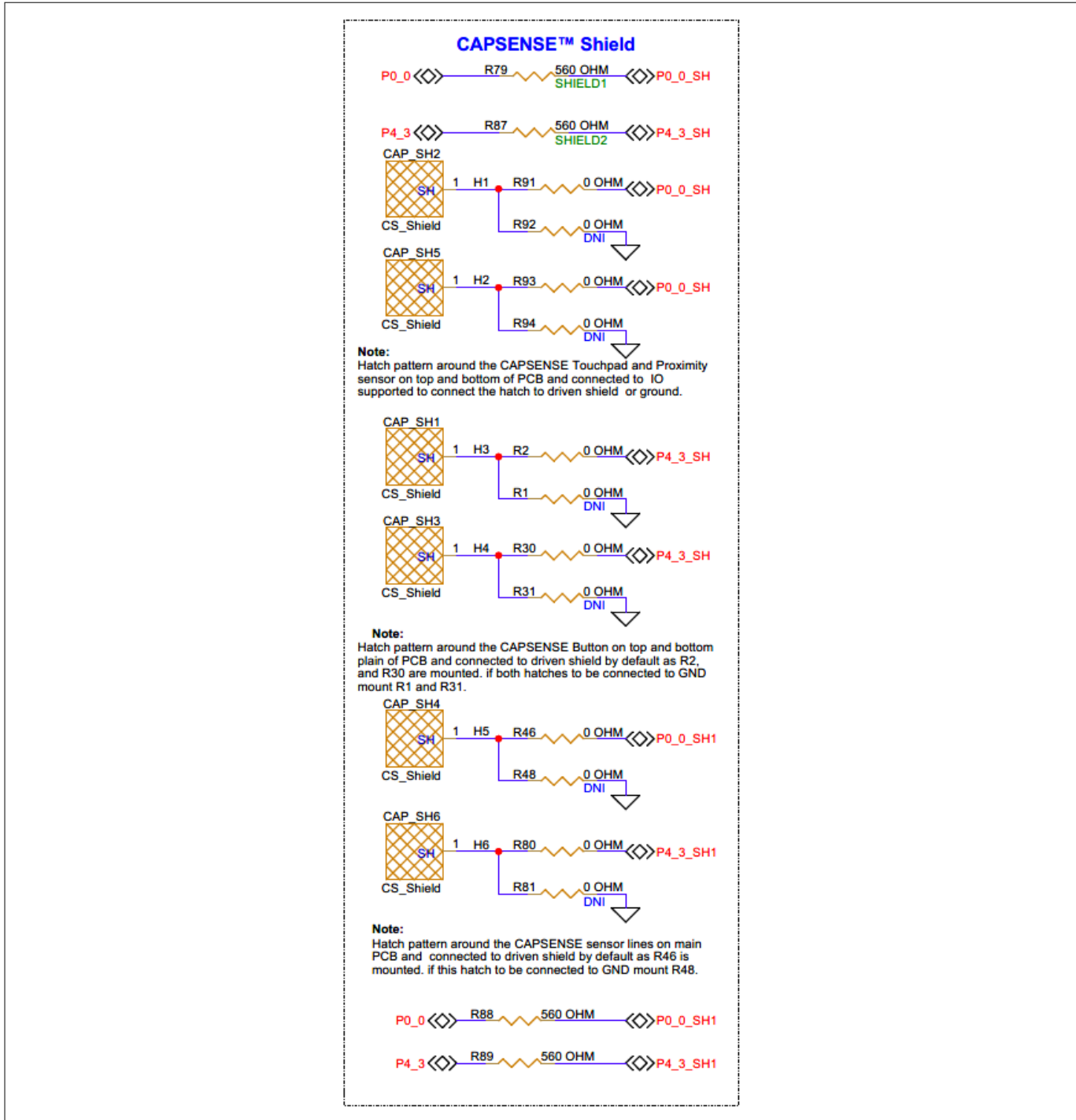
Figure 40 Schematic of driven shield configurations
