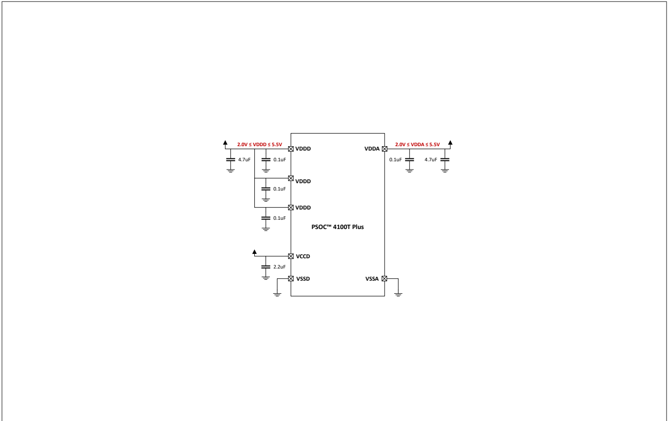
Figure 20 PSOC™ 4100T Plus MCU schematic with 2.0 V to 5.5 V external supply
