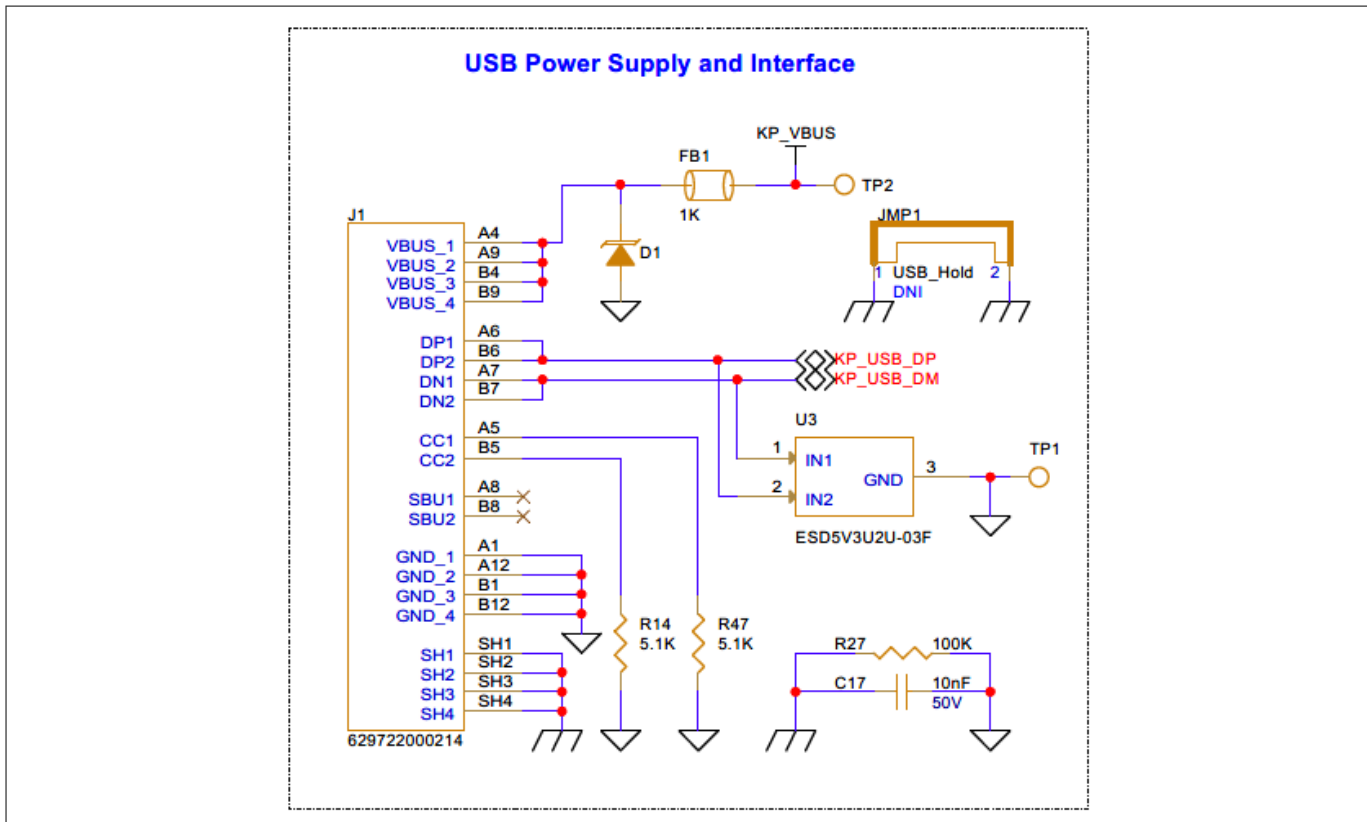
Figure 32 USB Type-C connector (J1) and ESD protection (D1, U3) schematic
