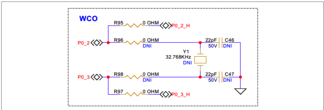
Figure 51 Schematic of rework regions to enable the WCO for the PSOC™ 4100T Plus device
