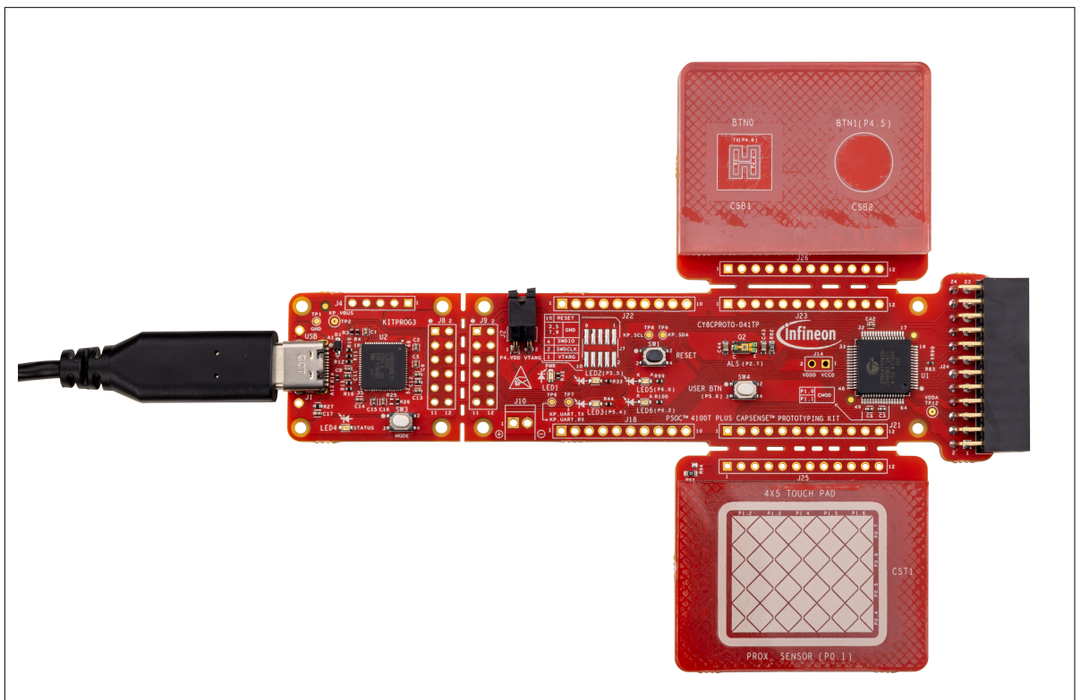
Figure 12 Connect the USB cable to the USB connector on the board
