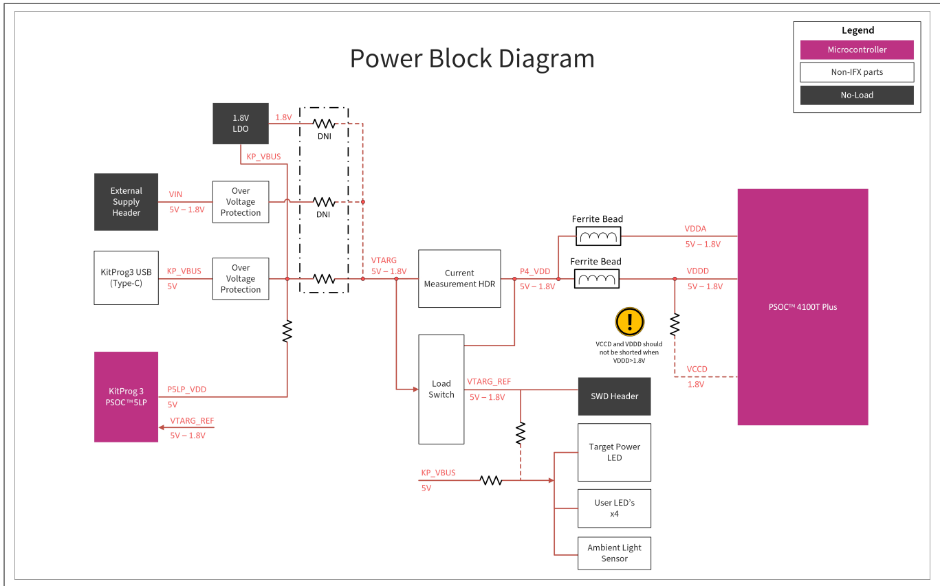
Figure 31 Power block diagram
