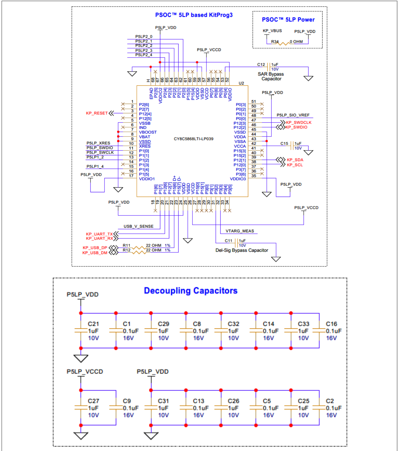
Figure 28 Schematic of PSOC™ 5LP-based KitProg3
