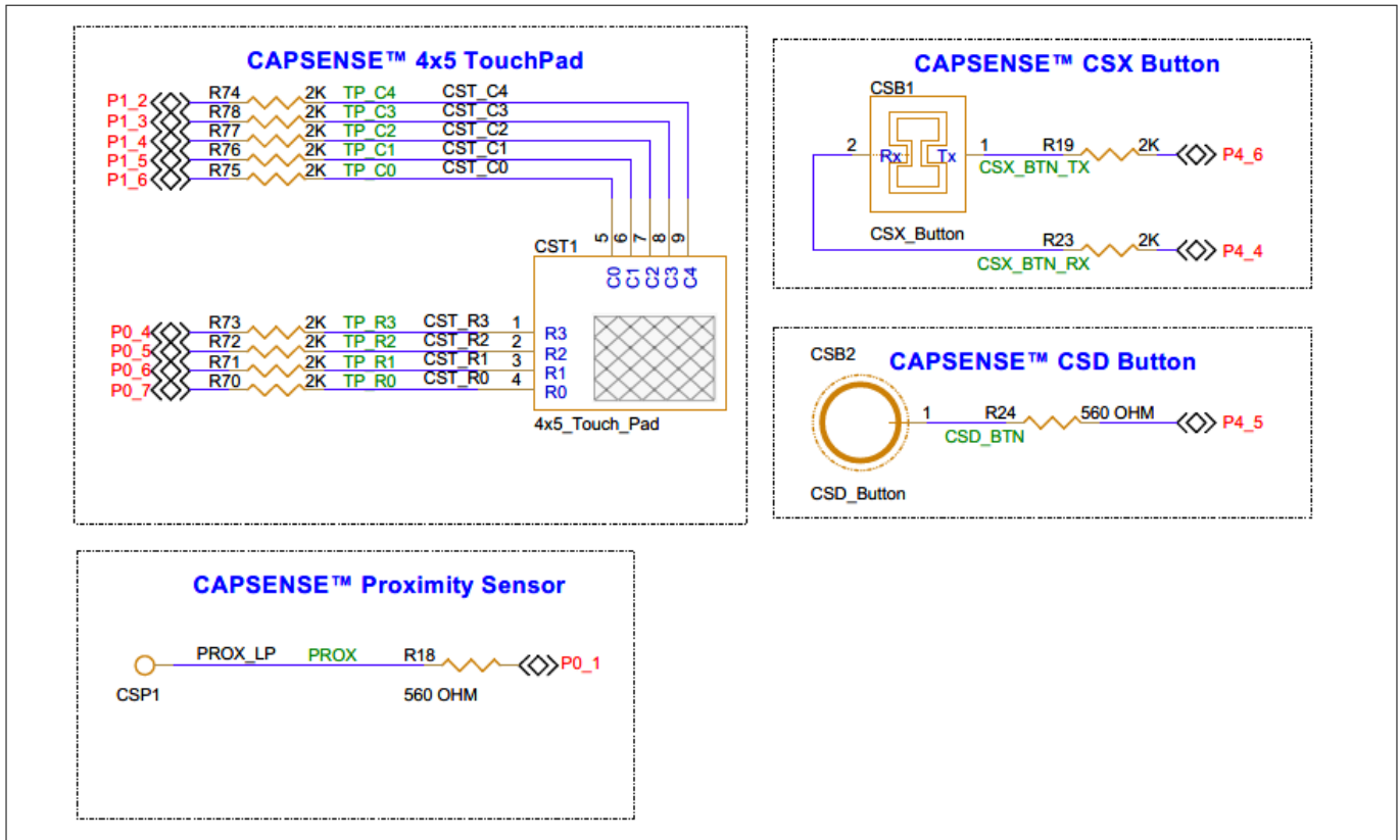
Figure 37 Schematic of capacitive sensing widgets
