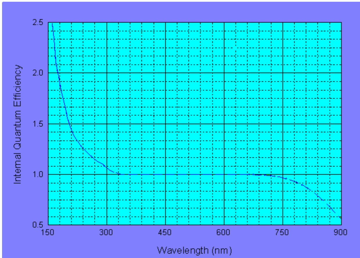
Fig. 1: Internal quantum efficiency of UVG photodiodes
