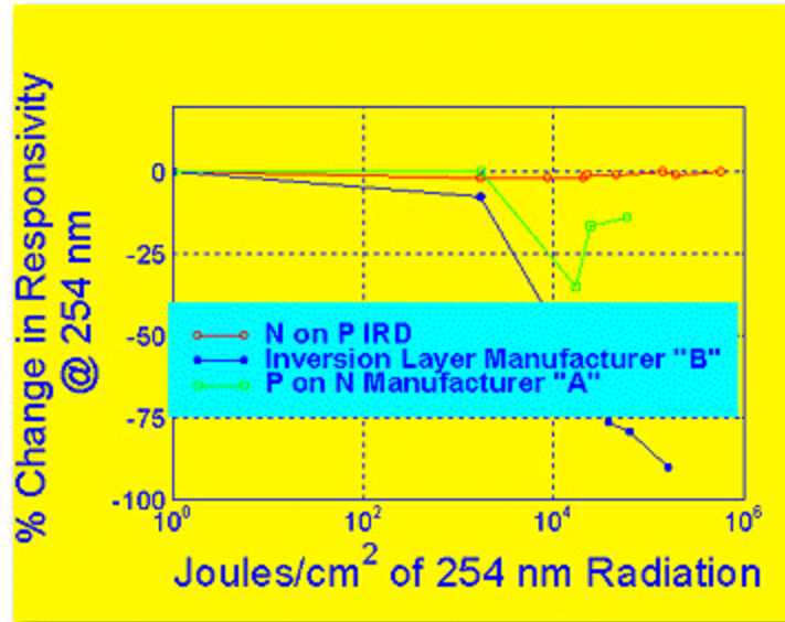
Fig. 2: Stability of a UVG series diode compared to other types of diodes after exposure to 254 nm radiation
