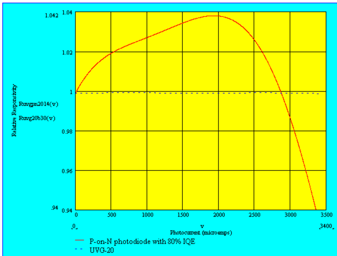
Fig. 2: Linearity of P-on-N photodiode with 80% internal quantum efficiency and UVG-20 photodiode with 100% internal quantum efficiency.
