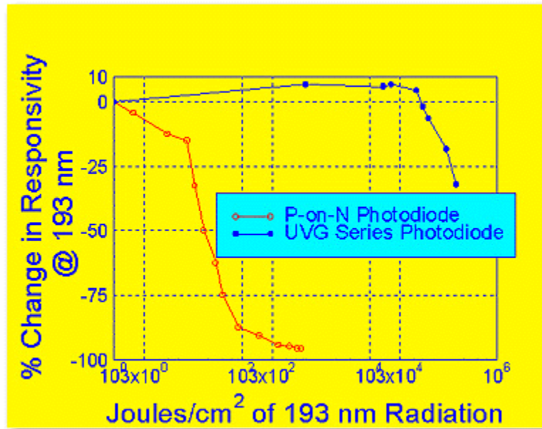
Fig. 3: Stability of a UVG series diode compared to p-on-n diode when exposed to 193 nm radiation.
