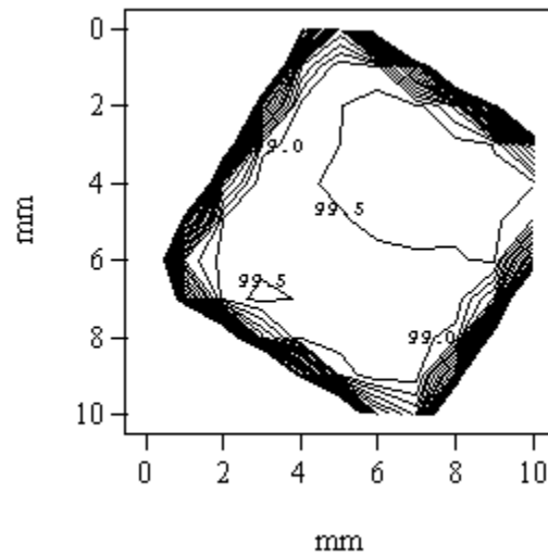
Fig. 1: Uniformity of IRD photodiode at 240 nm [1].
