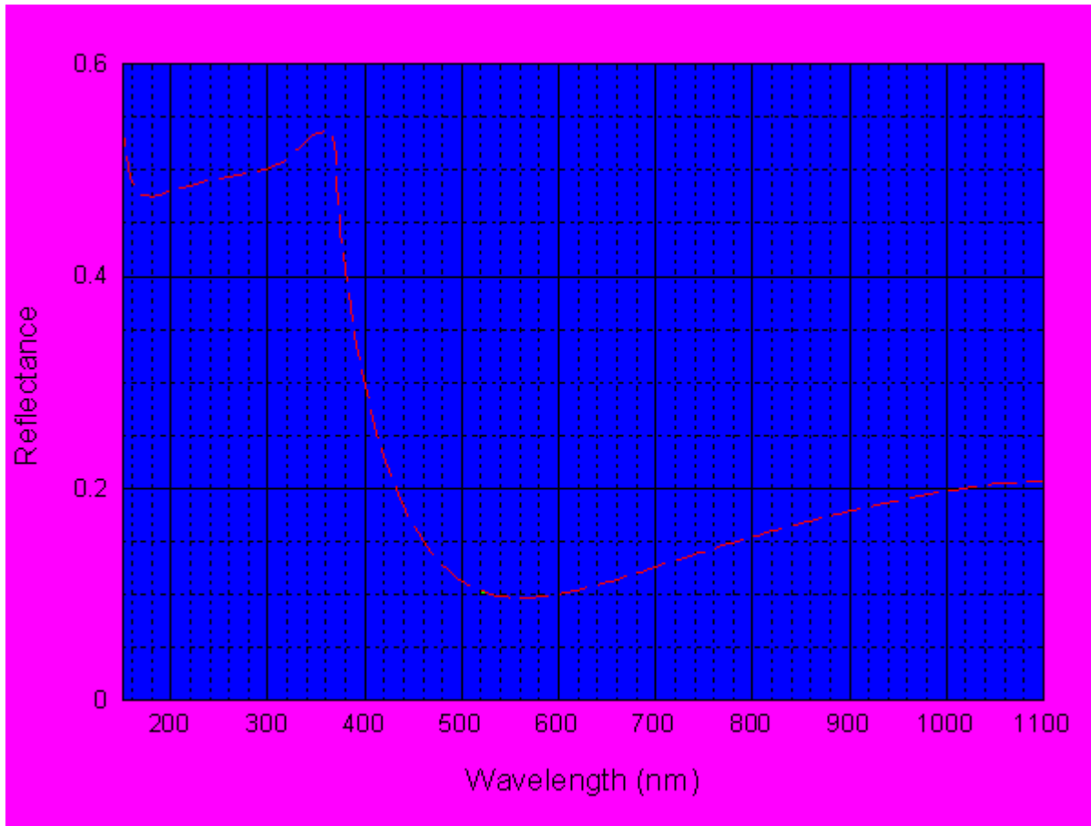
Fig. 2: Typical reflectance of UVG series photodiodes.
