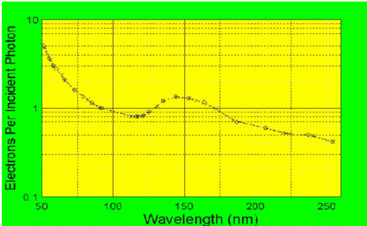
Fig. 1: Quantum efficiency of UV-enhanced photodiodes with 60 Å oxynitride passivating front window. O Before exposure, X after exposure to 100% relative humidity for 4 weeks.
