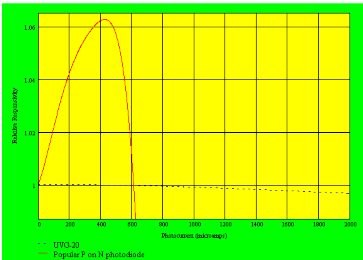
Fig. 3: Linearity of UVG-20 photodiode and widely used P-on-N photodiode when tested at 980 nm with no reverse bias
