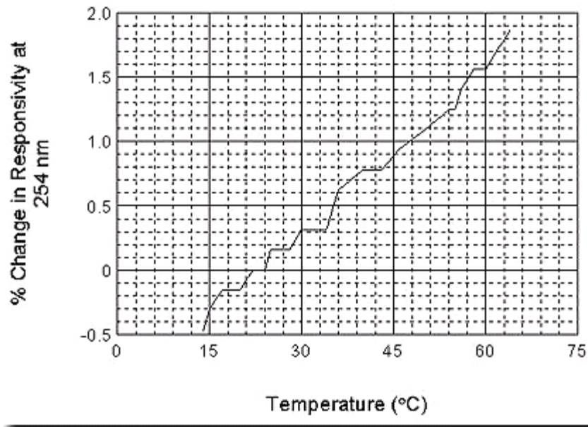
Fig. 2: Change in 254 nm responsivity of UVG photodiodes with temperature.
