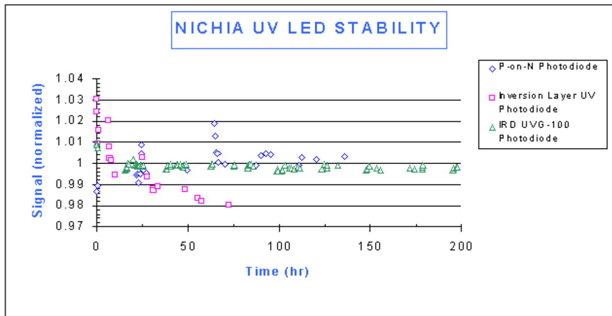
Fig. 4: Nichia 378 nm LED stability measured with p-on-n, inversion layer, and the UVG-100 photodiodes [7].
