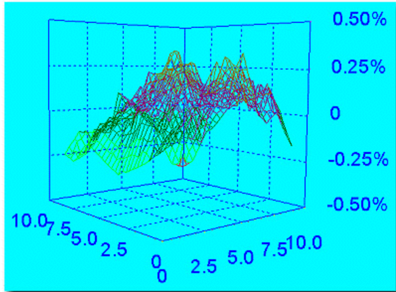
Fig. 1: Uniformity of UVG-100 photodiode at 254 nm.
