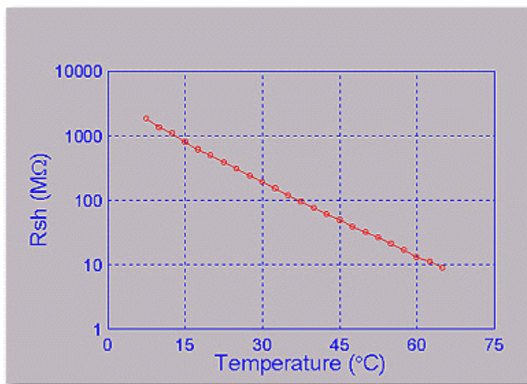
Fig. 3: Change in shunt resistance of UVG photodiodes with temperature.
