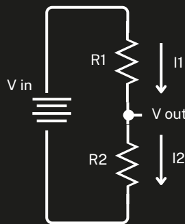
Voltage Division
