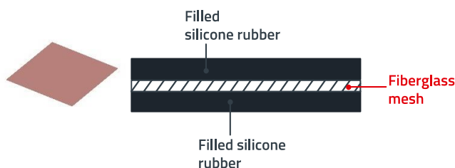
Figure 1: WE-TINS cross-section
