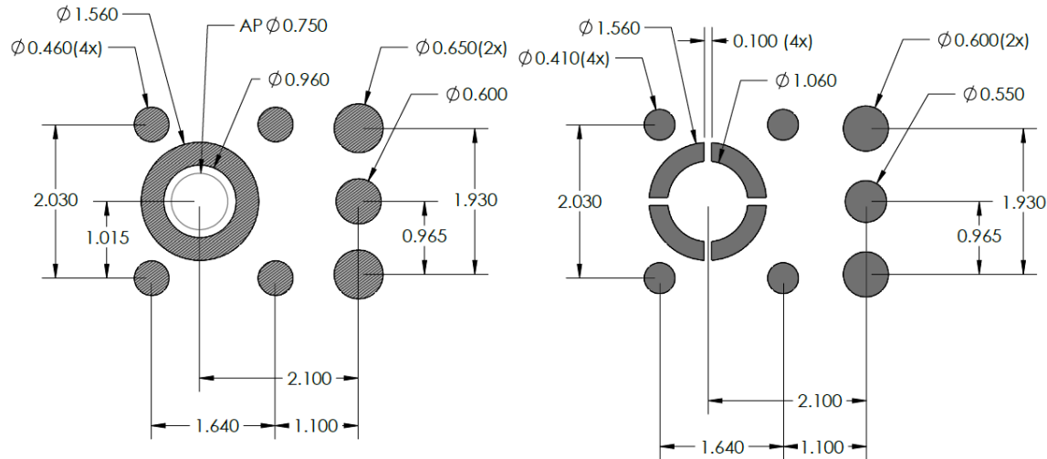
Figure 2: VM1010/VM2000 PCB land pattern (left) and solder stencil pattern (right)
