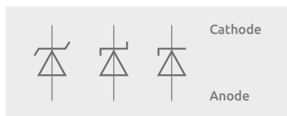
Figure 39 | Common symbols for a Zener diode.
