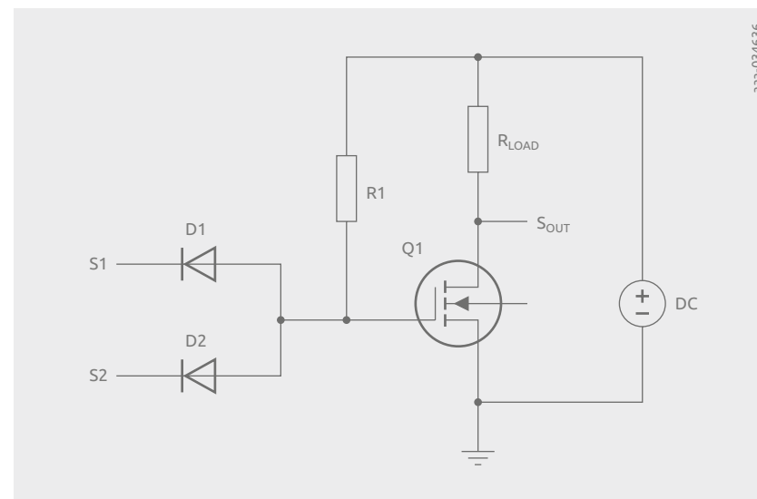
Figure 117 | Diodes AND function with FET switch added
