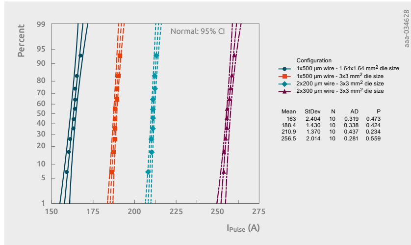
Figure 50 | Probability Plot of D²PAK for different Bonding technologies.
