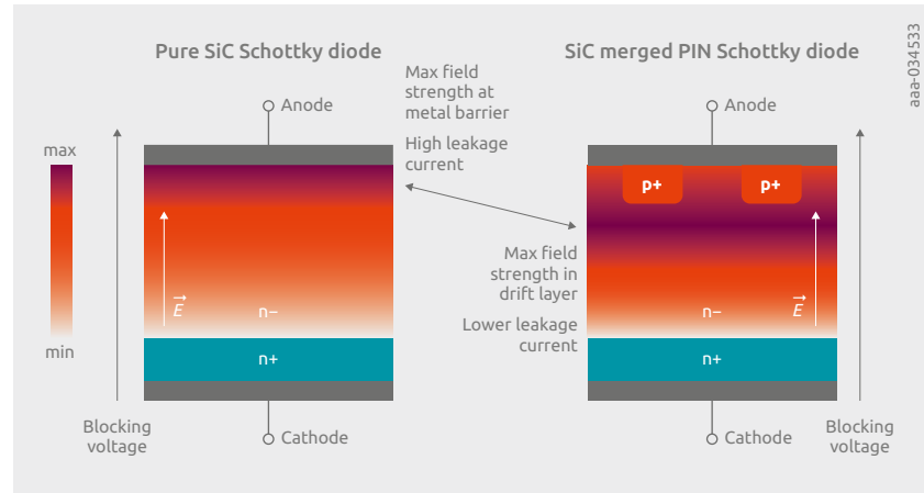
Figure 30 | Comparison of e-field distribution of pure Schottky diodes & MPS at reverse bias.
