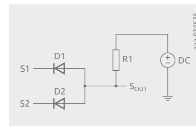
Figure 116 | Diodes AND function.
