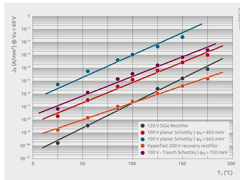
Figure 12 | Dependence of the leakage current density (normalized leakage current with respect to the active area) at a reverse bias voltage of –60V on the junction temperature for different 100V technologies.
