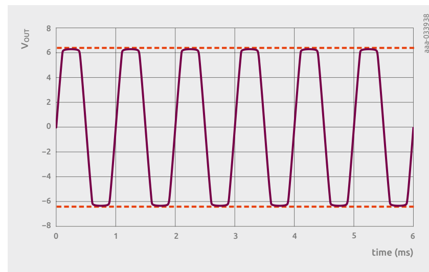
Figure 110 | Symmetrical clipping of 1 kHz sine wave with BZT52H-B5V6.
