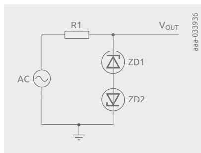
Figure 109 | Example for level clipping of AC voltage by Zener diodes.
