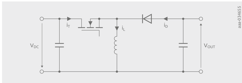
Figure 137 | Schematic of a buck-boost converter.
