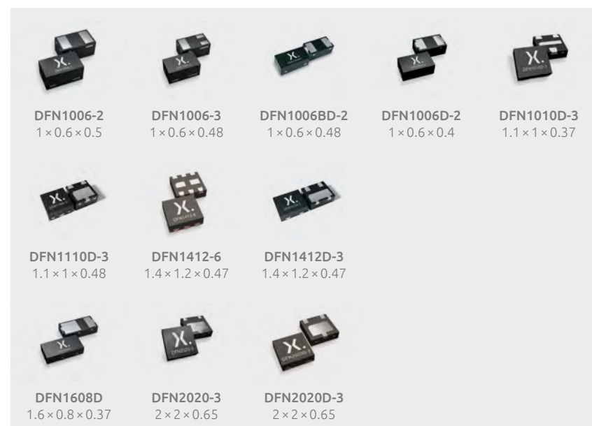
Figure 94 | Table of Nexperia diode DFN packages with outline and dimensions in mm.
