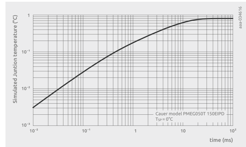
Figure 90 (below) | Simulated junction temperature vs. time for an applied power of 1W to PMEG050T150EIPD. Solder point temperature set at 0°C.
