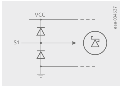
Figure 118 | Switching diodes applied as input protection.
