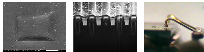
Figure 98 | Potential failure modes during device operation: crystal defects (left), incomplete trench (center) and lifted bond due to intermetallic corrosion.
