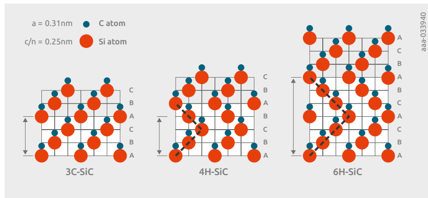
Figure 24 | SiC polytypes
