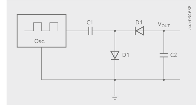
Figure 119 Voltage inverter with charge pump approach.
