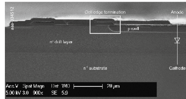
Figure 3 | SEM picture showing the cross section of a recovery rectifier. The sample has been etched in order to decorate the different doping regions.
