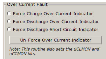
FIGURE 48. OVERCURRENT FAULT DEMO OPTIONS
