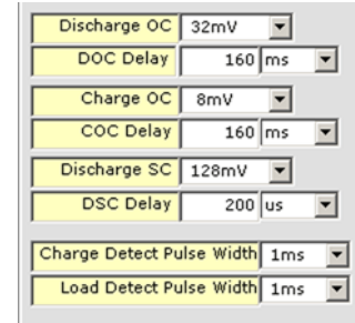
FIGURE 32. CURRENT LIMITS
